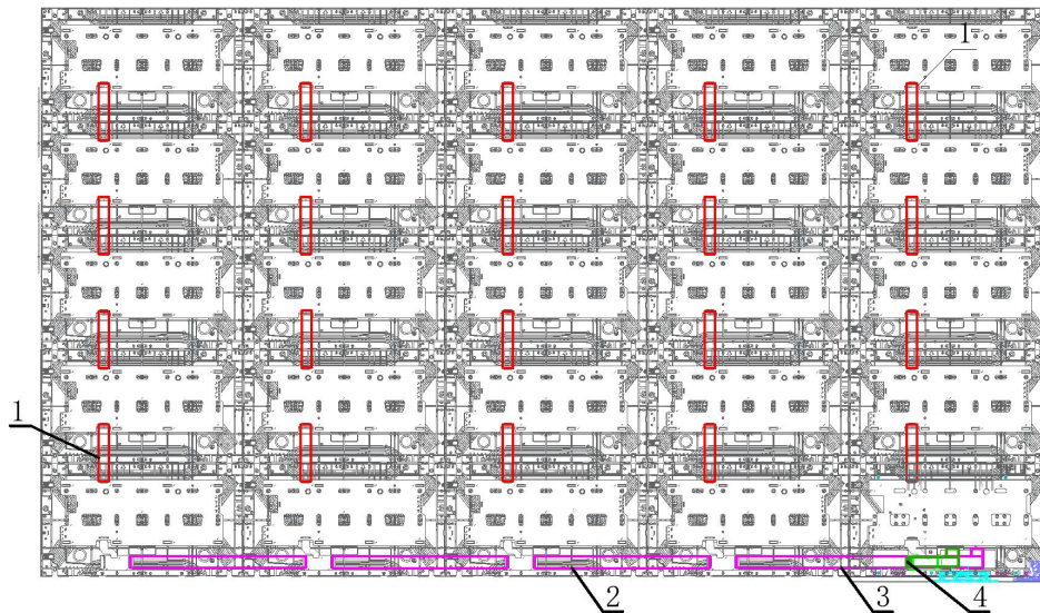
Signal wiring diagram
